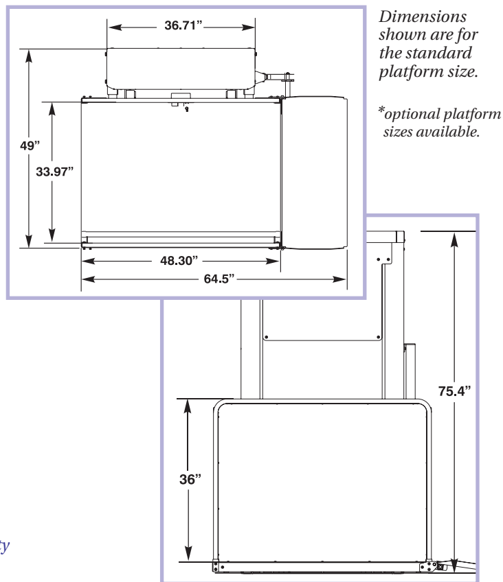
Dimensions shown are for the model VPL-3153
